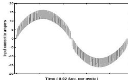
Figure. 3 Inductor current made of charging and Discharging phases
