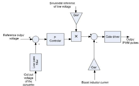
Figure.2 PWM controller with two feedback loops
