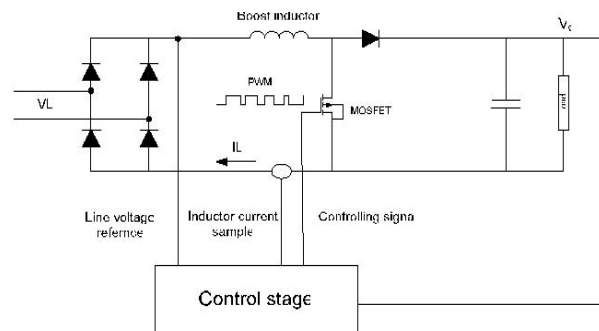
FIG 1) Dual loop PWM controller circuit
