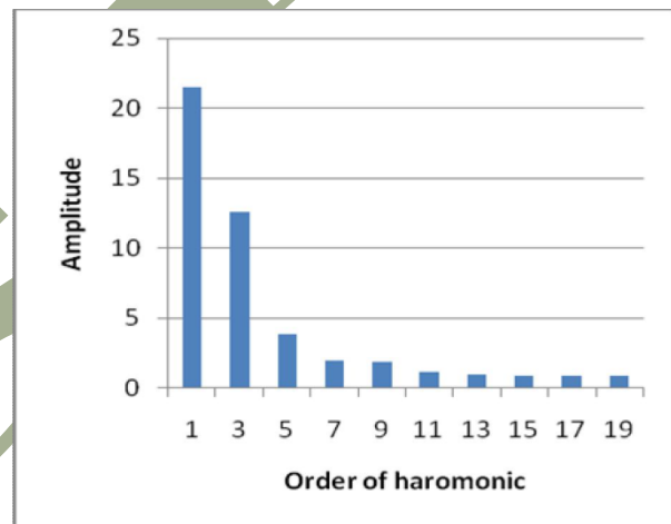
FIG 6 Odd harmonic plot before input current shaping.
