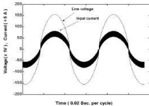
Figure. 5: Shows the input current plotted over the line voltage.
