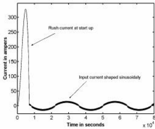
Figure. 4 Shows the input line current after input-current Shaping
