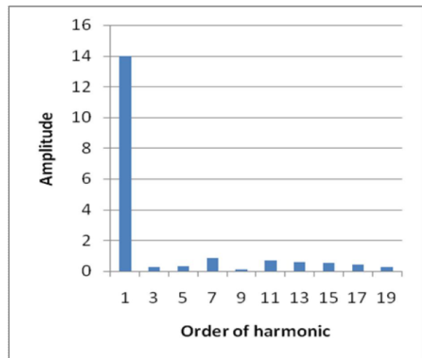
FIG 7 Odd harmonic plot after input current shaping.
