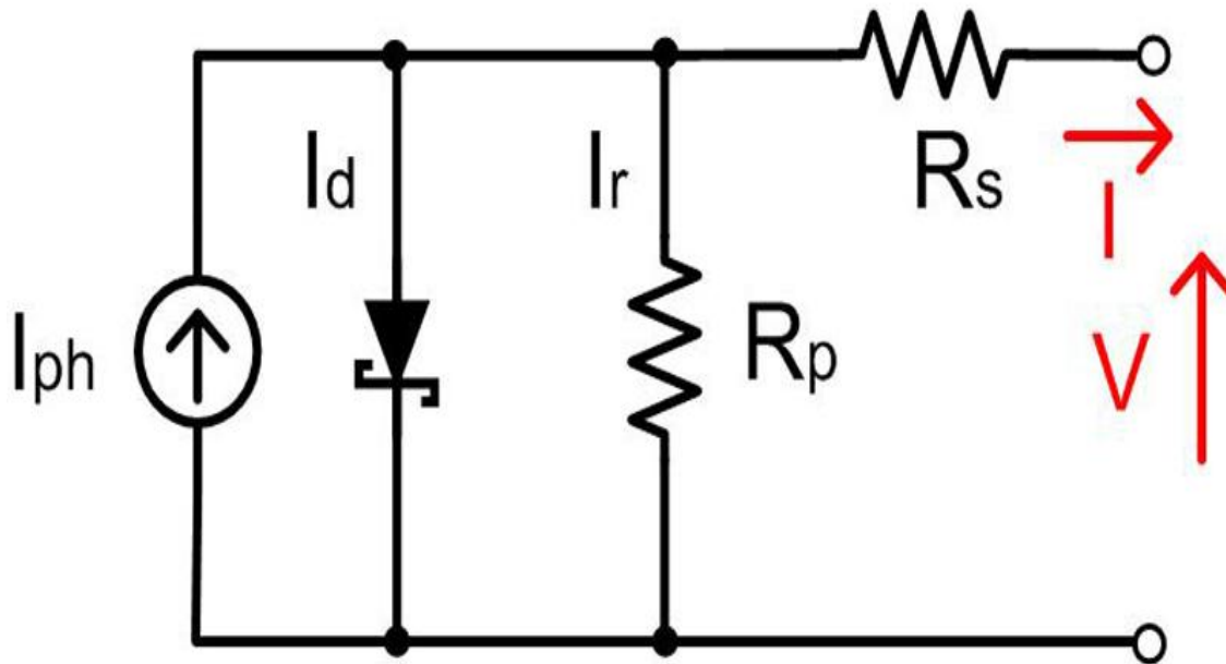
Fig 2 PV Model
