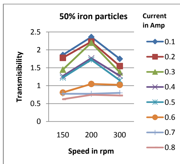
Graph 8.3 Transmissibility v/s speed for sample 3
