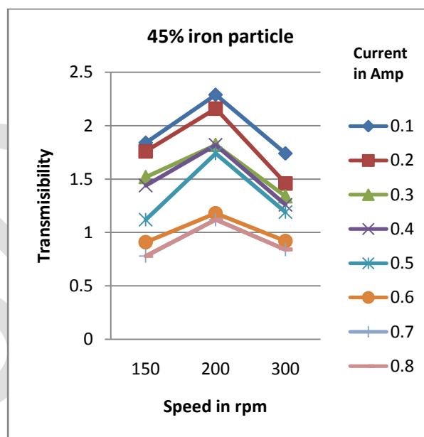
Graph 8.2 Transmissibility v/s speed for sample 2
