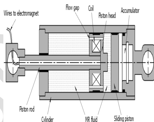
Fig.1.1 Magneto rheological Damper
