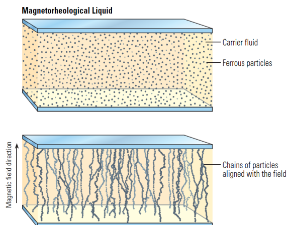
Fig 1.2 chain like structure formation in controlable fluid
