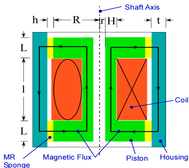
Fig.3.1 Dimensions of MR Fluid Damper
