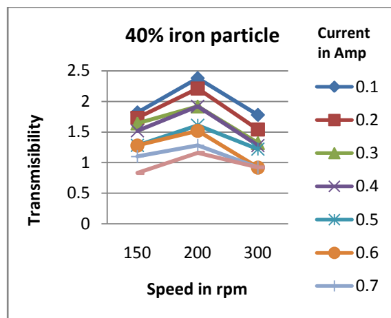
Graph 8.1 Transmissibility v/s speed for sample1
