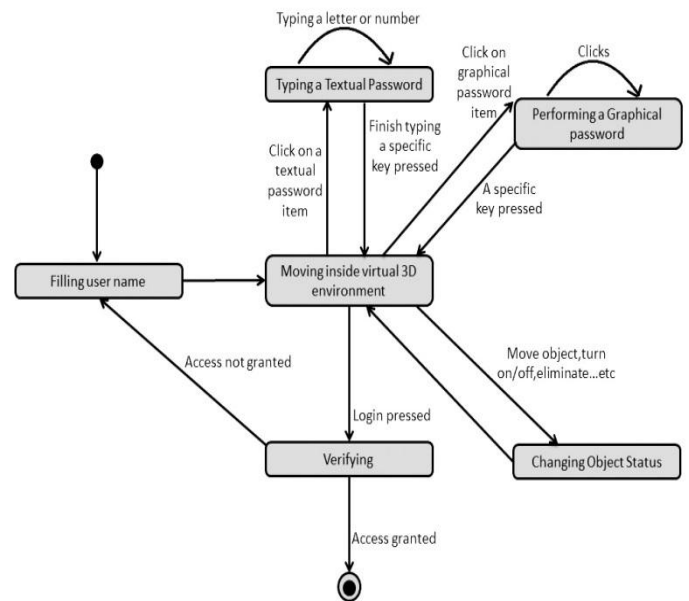
Fig. 3 State diagram for creating 3D password
