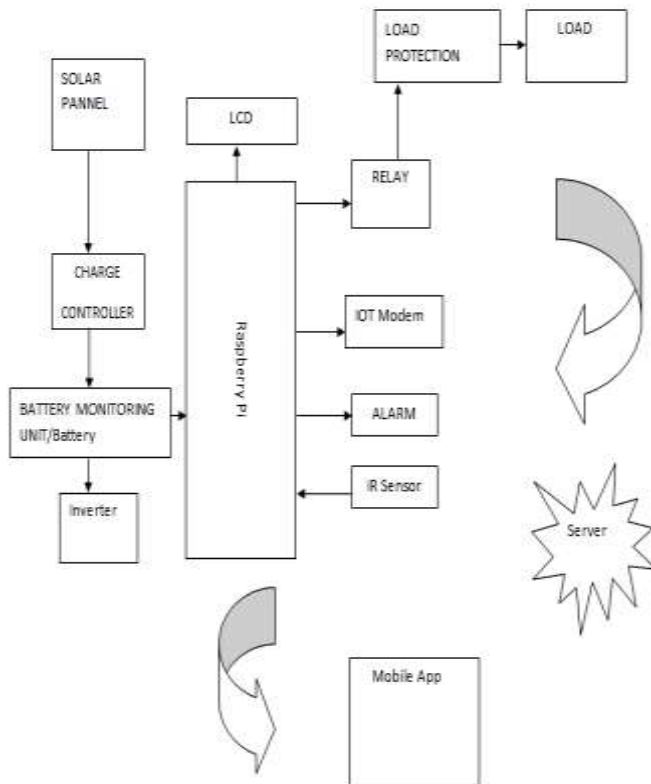
Fig 2. Block diagram of IoT based smart inverter using Raspberry pi
