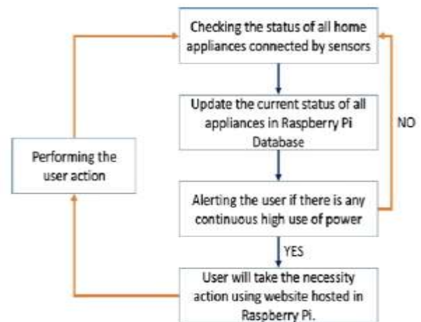
Fig 4. Algorithm showing raspberry pi working system
