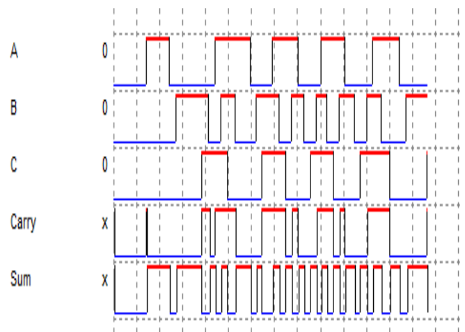
Figure IV: Simulated Overall Timing Diagram of DSCH 10T Full Adder Circuit
