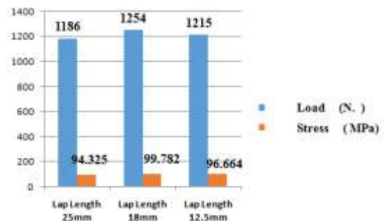
Fig. 15 Comparison value of rivet joint
