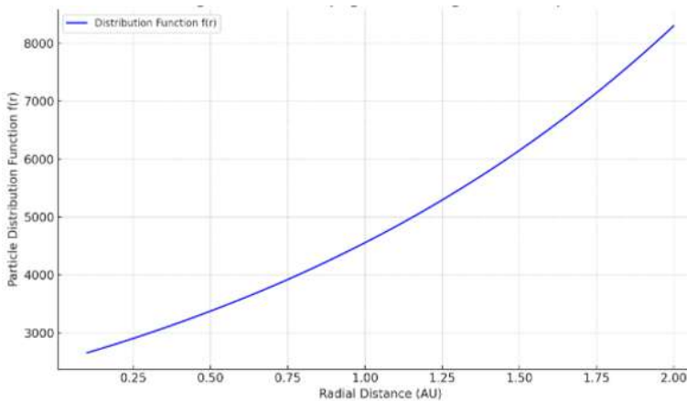
Figure 8: energetic particle distribution function
