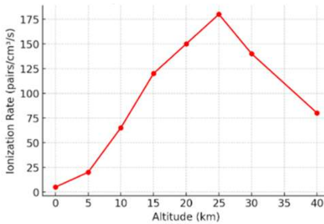
Figure 3: Figure 3. Ionization rates vs altitude from GEANT4-like lookup, for GCR and SEP spectra.
