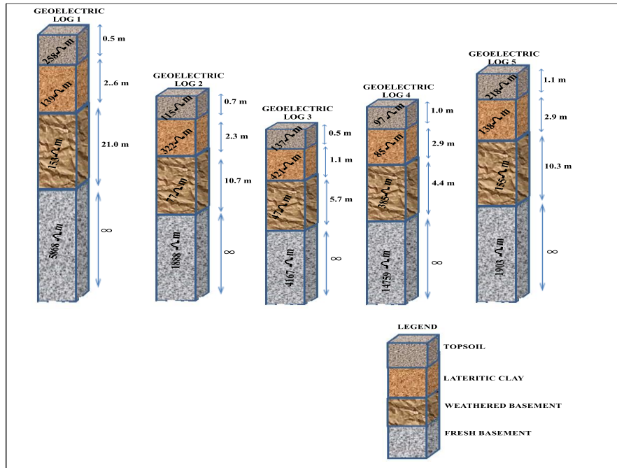
Figure 3: Geoelectric logs
