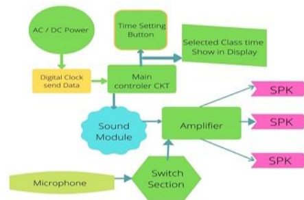
Fig. 1. Flow Chart of the Proposed System.
