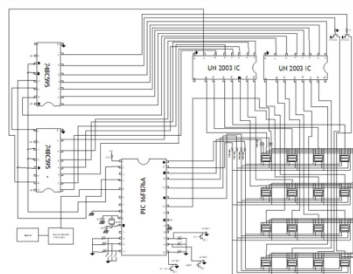
Fig. 6. Circuit Diagram of Control Section
