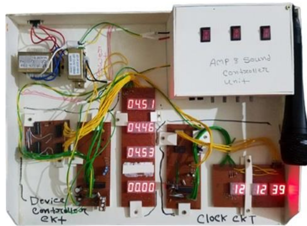
Fig. 7. Real time Project circuit.
